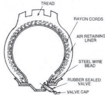
Fig. Tubeless Tyre
