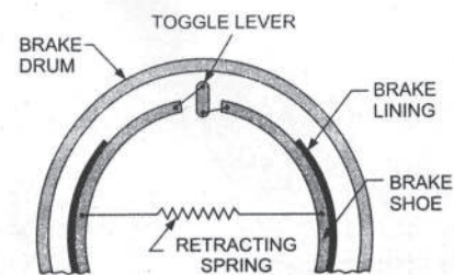
Toggle lever is used to expand shoes.
