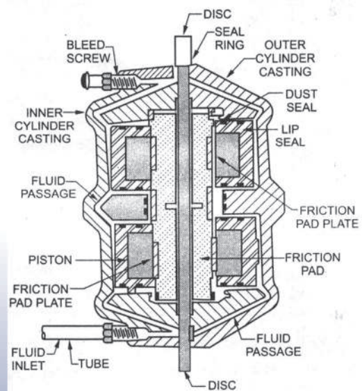
Caliper type disc brake.
