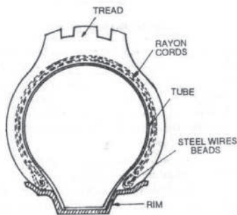
Fig. Traditional Tube Tyre
