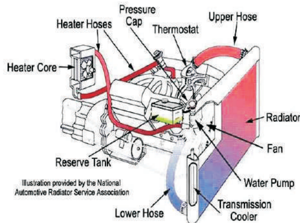
Fig : Automobile Cooling System
