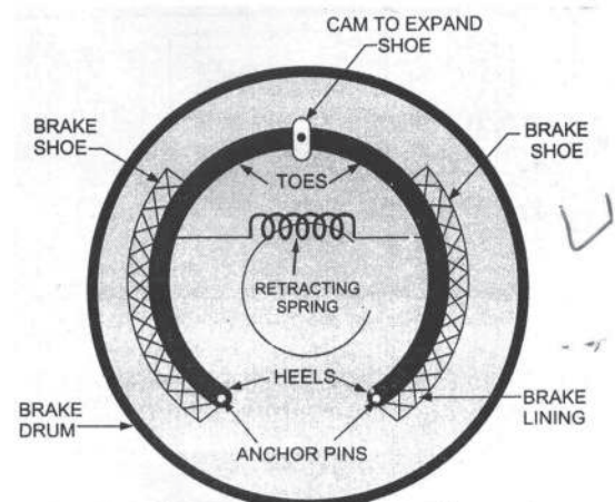
Shoe mounting in an internal expanding brake (using Cam to expand shoes)
